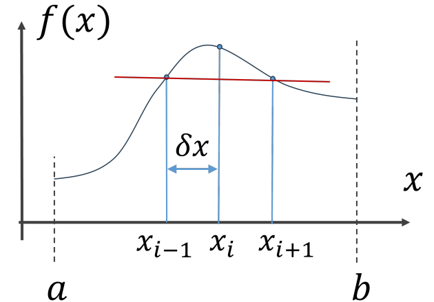
Central difference
