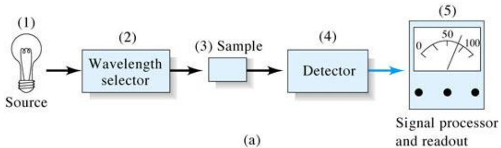
FIGURE 7-1 Components of various types of instruments for optical spectroscopy.
