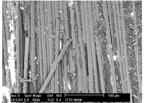
Fracture surface of the plain-weave S-2 glass fabric SC-15 epoxy composite
