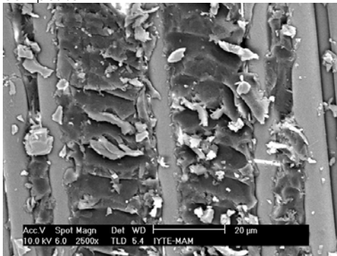
Fracture surface of the plain-weave S-2 glass fabric SC-15 epoxy composite
