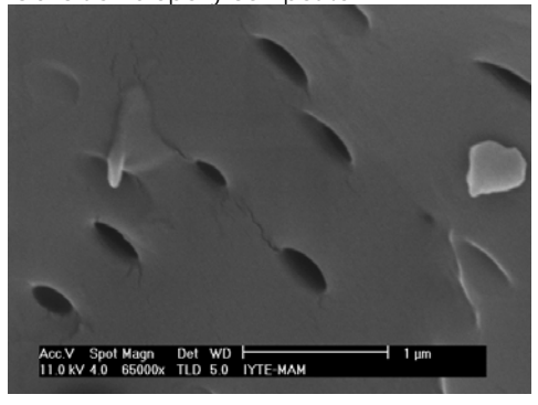
Fracture surface of the plain-weave S-2 glass fabric SC-15 epoxy composite, showing rubber particles
