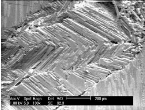
compression tested woven fabric S2-glass fiber reinforced vinyl ester composite
