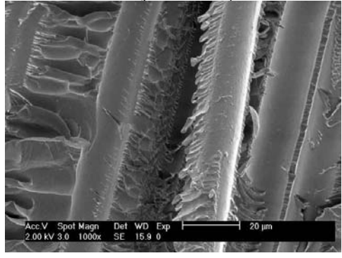
Fracture surface of the woven fabric S2-glass fiber reinforced vinyl ester composite
