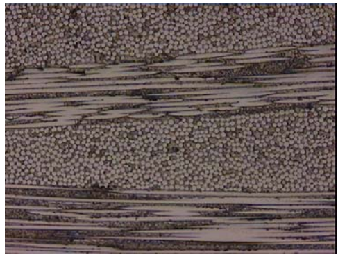
woven fabric S2-glass fiber reinforced vinyl ester composite
