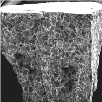
SiC particle reinforced Al 2 O 3 Ceramic Matrix Composite's fracture surface pictures at various magnifications in SiC and matrix (Al 2 O 3 and Al)
