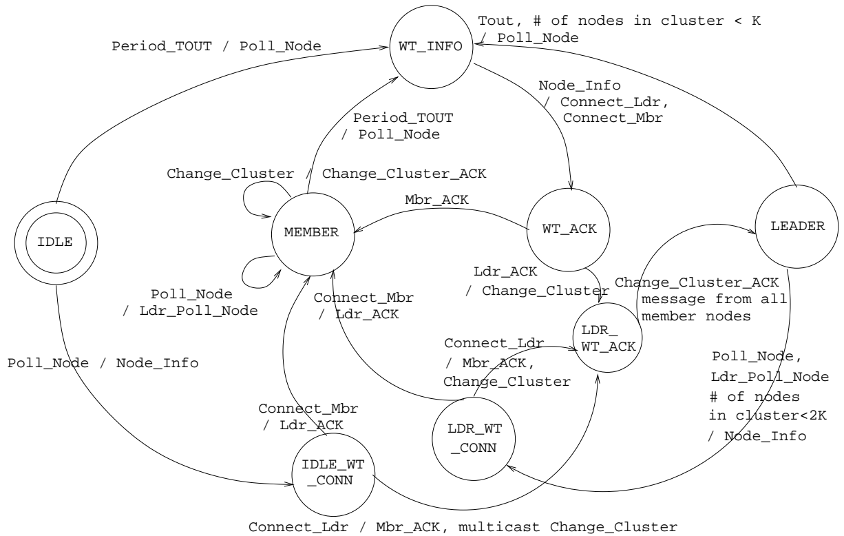
Figure 3.1. Finite State Machine of the Merging Clustering Algorithm
