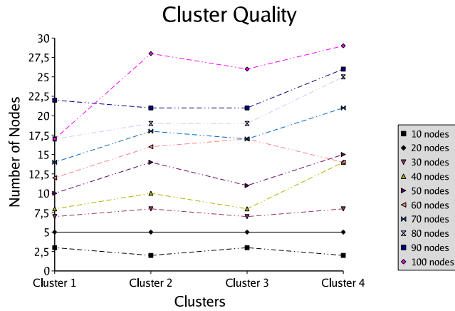
Fig. 6. Cluster Node Counts
