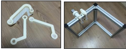
Fig. 6. Manipulator Links that are Printed oh Rapid Prototyper and the Aluminum Manipulator Frame
