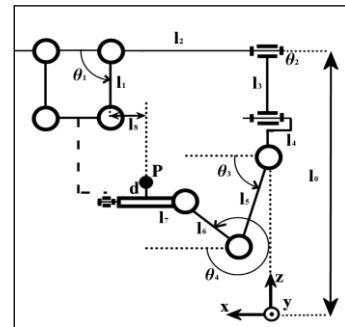
Fig. 4. Section View of the Cartesian Part of The Hybrid Manipulator from the x-z Plane
