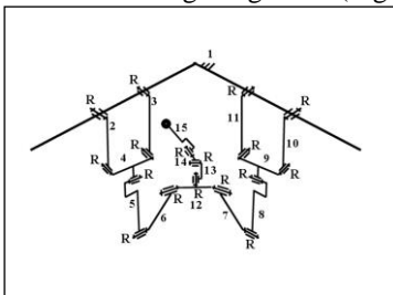
Fig. 3. Simple Kinematic Structure of Designed Hybrid Manipulator
